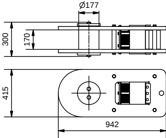
Anchor (1:20)
